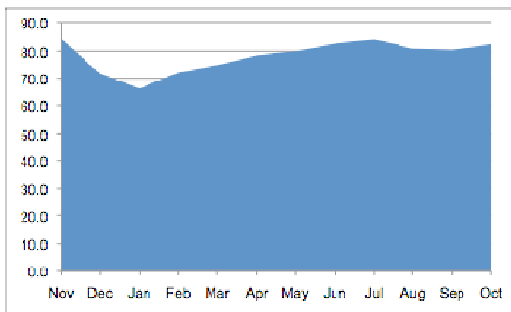
Figure 3.1 Hotel Room Occupancy Rate (%): Nov 2007 to Oct 2008
