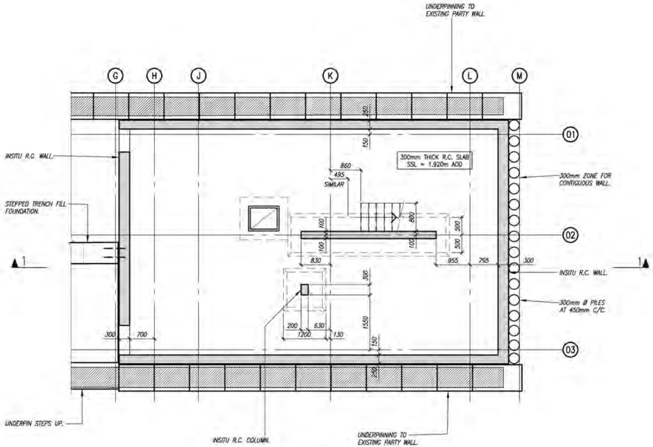
Basement Plan
